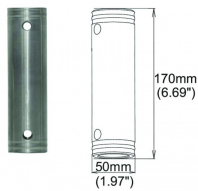
Spacer 170mm (6.69") female
