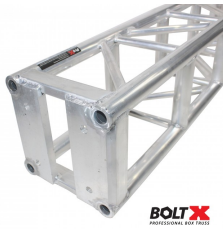
8 Ft. BoltX Bolted 12 Inch Professional Box Truss Segment | 3mm Wall SKU: XT-BT1208
