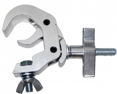
Aluminum Self-Locking M10 Clamp with Big Wing Knob for 2" Truss Tube Capacity 330 lbs. SKU: T-C12H
