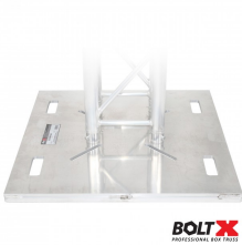
BoltX 24 inch Steel Aluminum Base Plate, Top Plate on a 1 inch Raised Frame for Bolted Box Truss SKU: XT-BTBP24A
